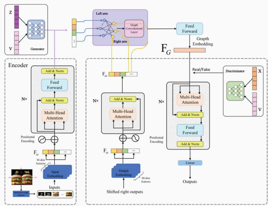
Figure 1. Overall algorithm framework
