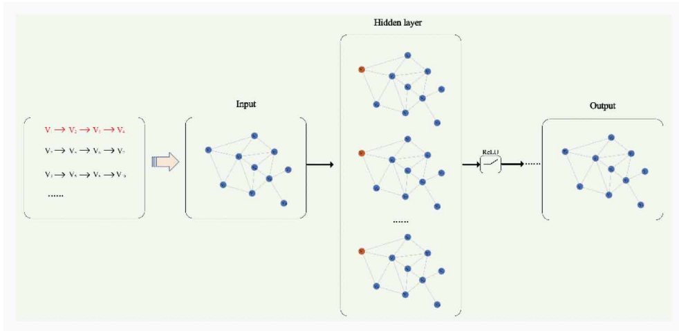
Figure 3. GNN
