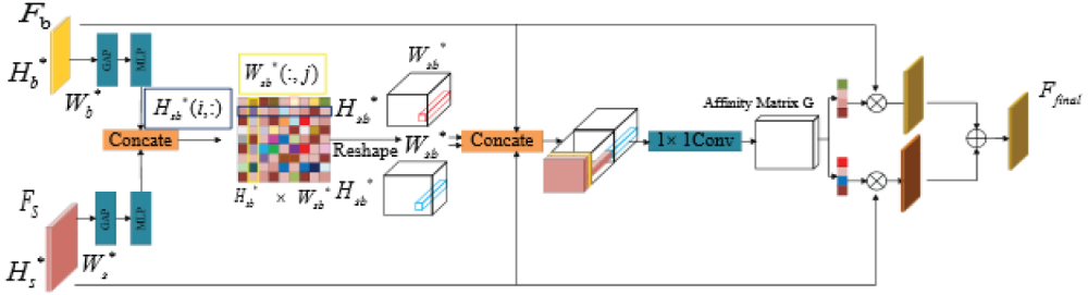
Figure 5. Detailed structure of the network module of SAWF
