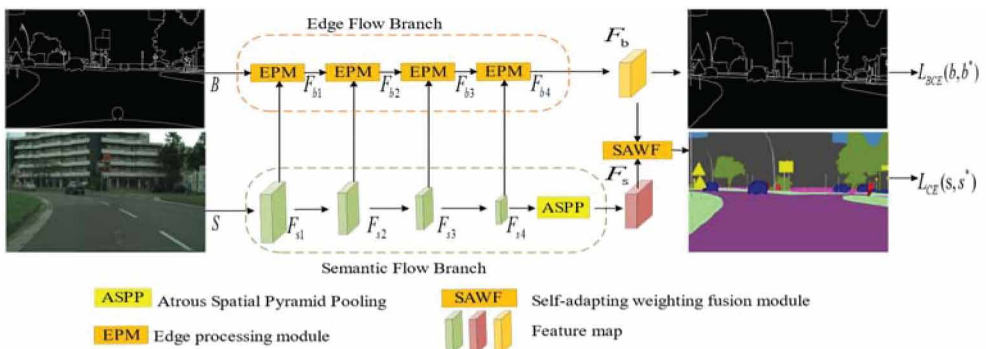
Figure 3. Detailed architecture of the overall framework of the EPSSNet model
