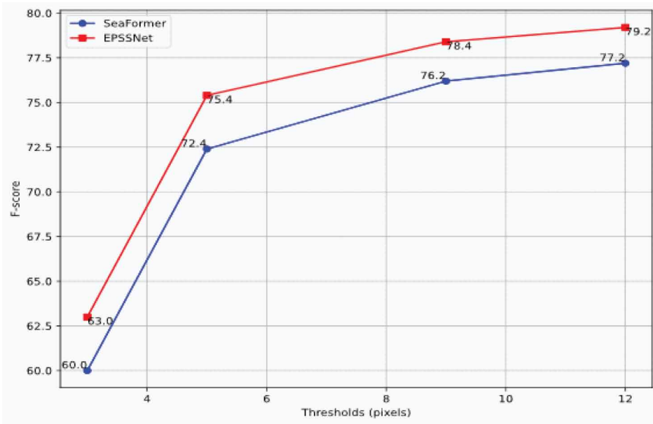
Figure 6. BloU metrics for EPSSNet vs. seaformer on the cityscapes dataset
