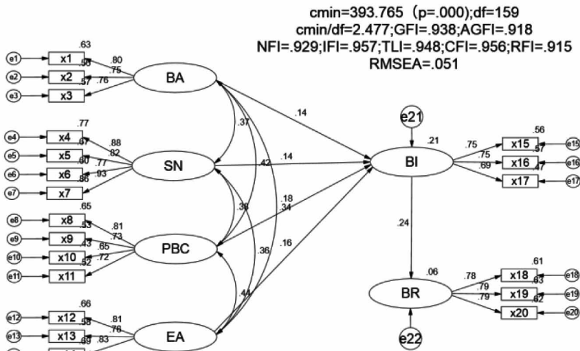
Figure 3. Obtained model and normalized path coefficients
