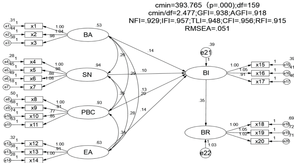
Figure 4. Obtained model and non-standardized path coefficients
