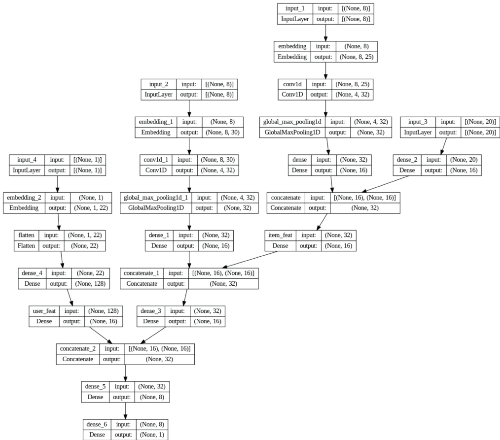
Figure 2. Flowchart of convolutional neural network model for feature extraction
