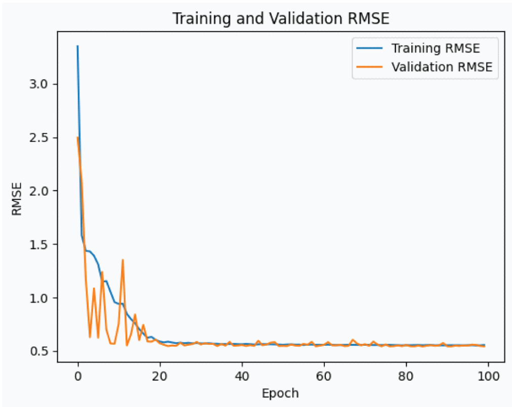
Figure 3. Training and validation root mean square error (RMSE)
