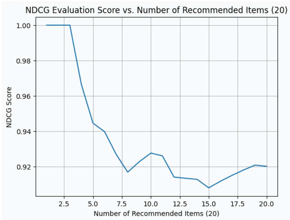
Figure 6. Normalized discounted cumulative gain (NDCG) evaluation score vs. number of recommended items
