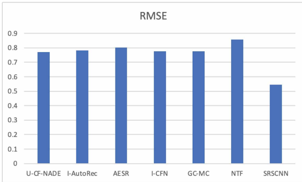
Figure 4. Performance comparison of each method based on RMSE
