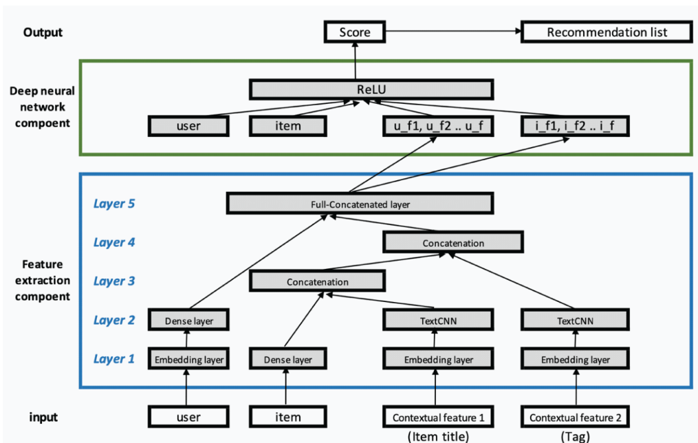
Figure 1. The proposed method (social recommender system based on convolutional neural networks)
