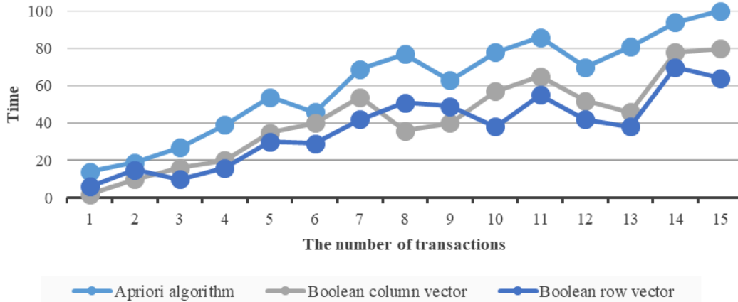
Figure 9. Performance comparison of Apriori algorithm and improved algorithm under different transaction numbers
