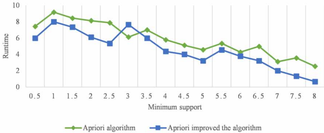
Figure 5. Minimum support curve before and after improvement
