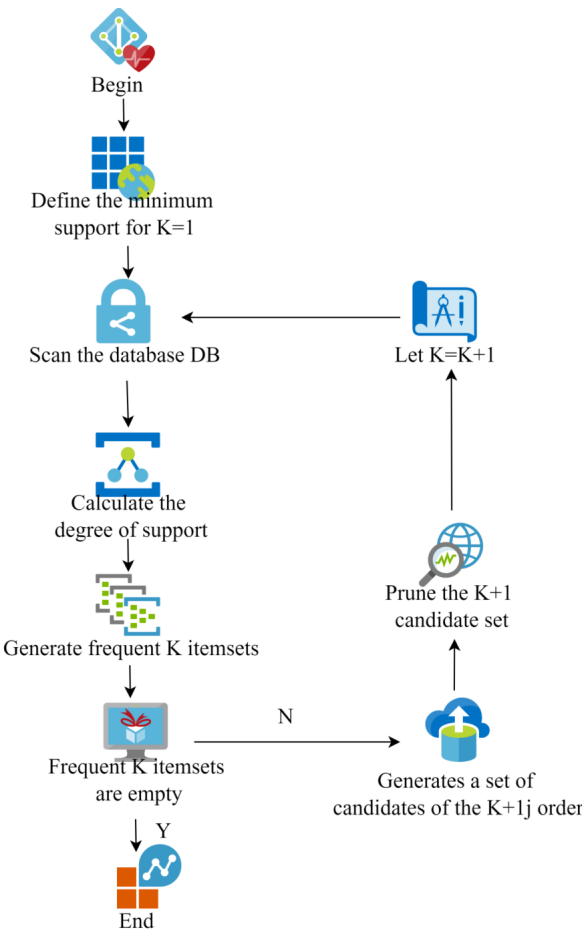
Figure 3. Apriori algorithm execution flow chart
