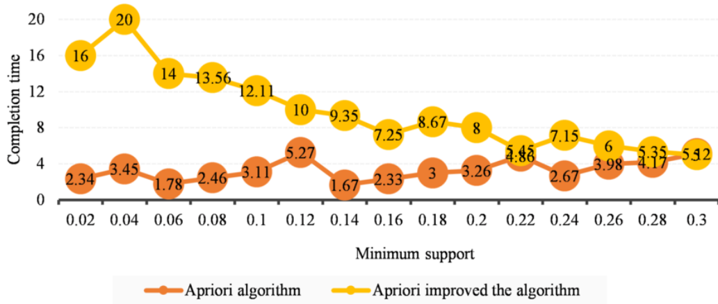
Figure 7. Comparison of experimental results of data sets
