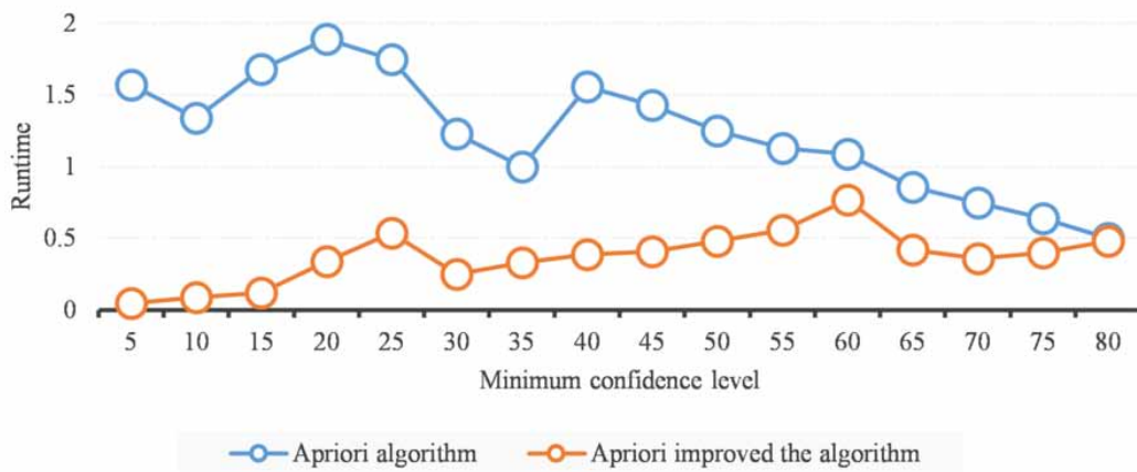
Figure 6. Minimum confidence curve before and after improvement
