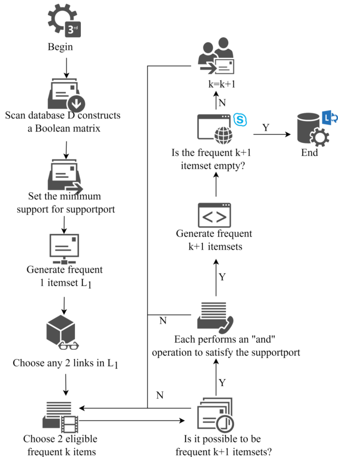
Figure 4. Flow chart of column vector arithmetic
