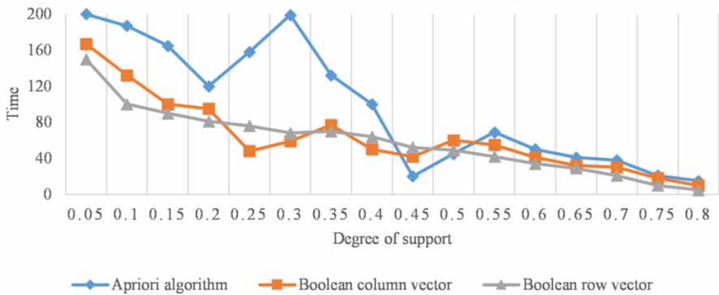
Figure 8. Performance comparison of Apriori algorithm and improved algorithm under different support levels
