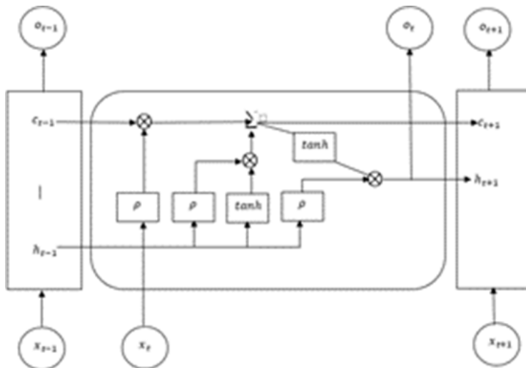
Figure 1. Schematic diagram of long short term memory
