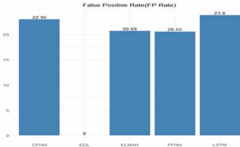
Figure 5. Classification analysis based on the false positive rate (FP Rate) criteria for diagnosis of cardiovascular disease
