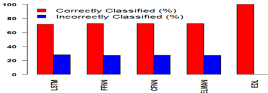
Figure 9. Comparison of classification accuracy
