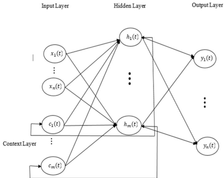
Figure 2. Structure of ELMAN neural network
