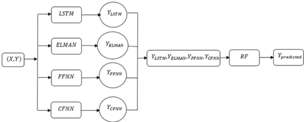
Figure 3. Schematic diagram of ensemble deep learning
