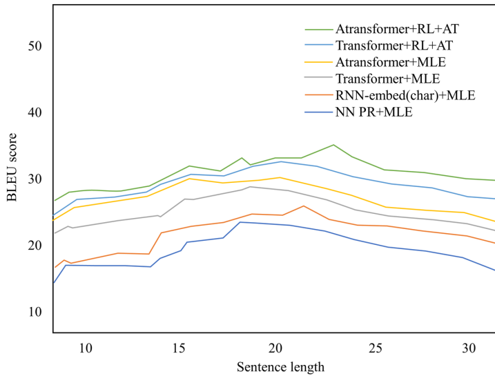
Figure 5. Comparison of BLEU scores of different models with sentence length
