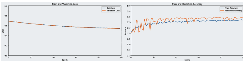
(e) CNN-Nadam- DS_1
