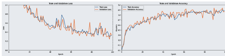
(a) CNN-Adam - DS_4
