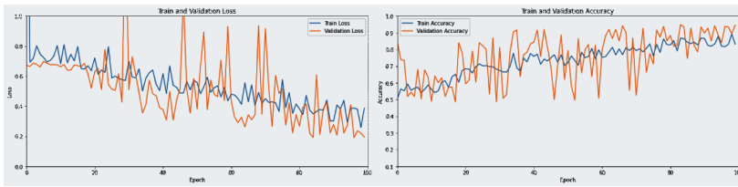
(a) CNN-Adam- DS_1
