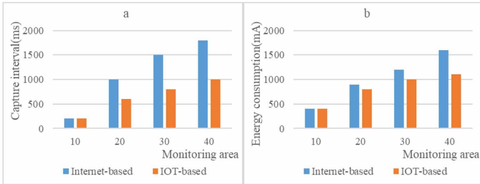
Figure 10. Capture time interval and energy consumption test chart
