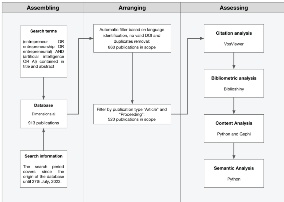
Figure 1. SPAR-4-SLR methodology
