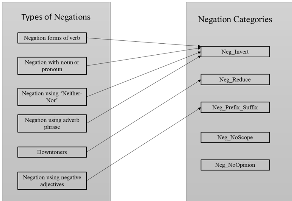
Figure 1. Types of negations and their mapping to negation categories
