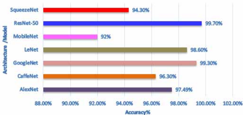
Figure 13. Chart showing the comparison of various architecture in plant disease detection
