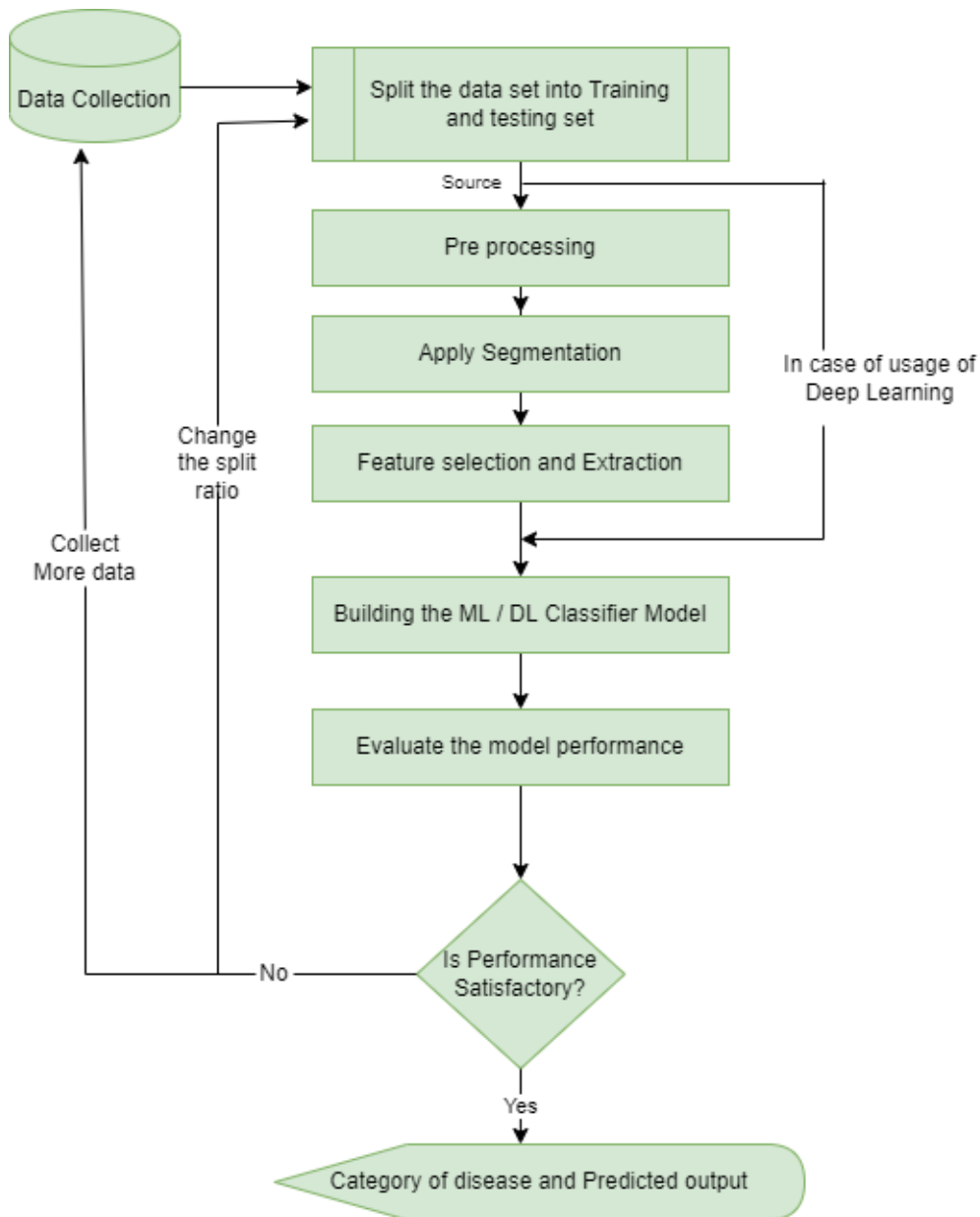
Figure 2. General Framework for Plant disease detection
