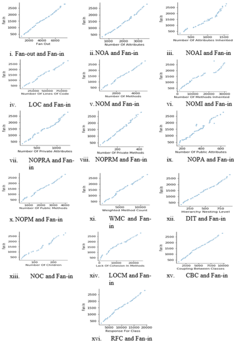
Figure 1. Fan-in Metric Correlation against Other Metrics
