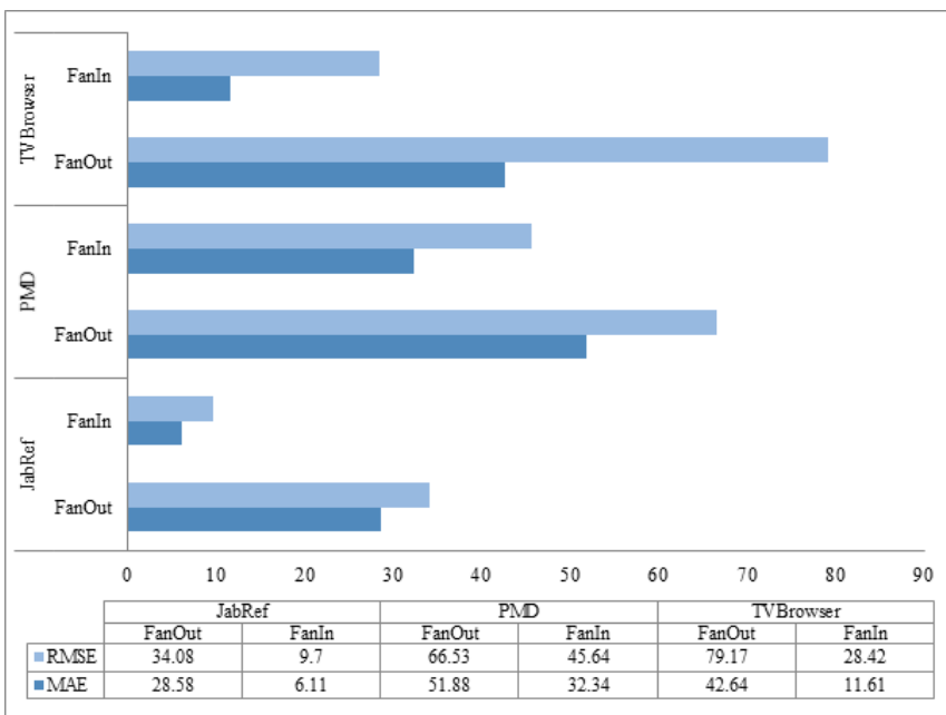
Figure 9. Accuracies of the model for each dataset
