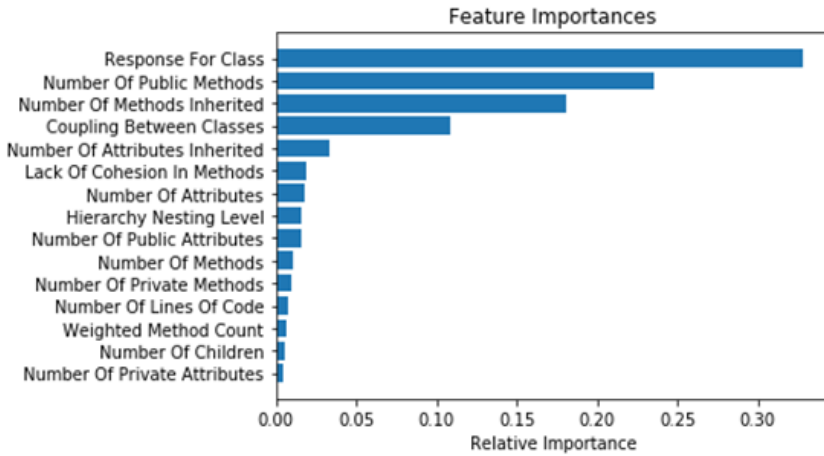
Figure 2. Relative Importance Chart
