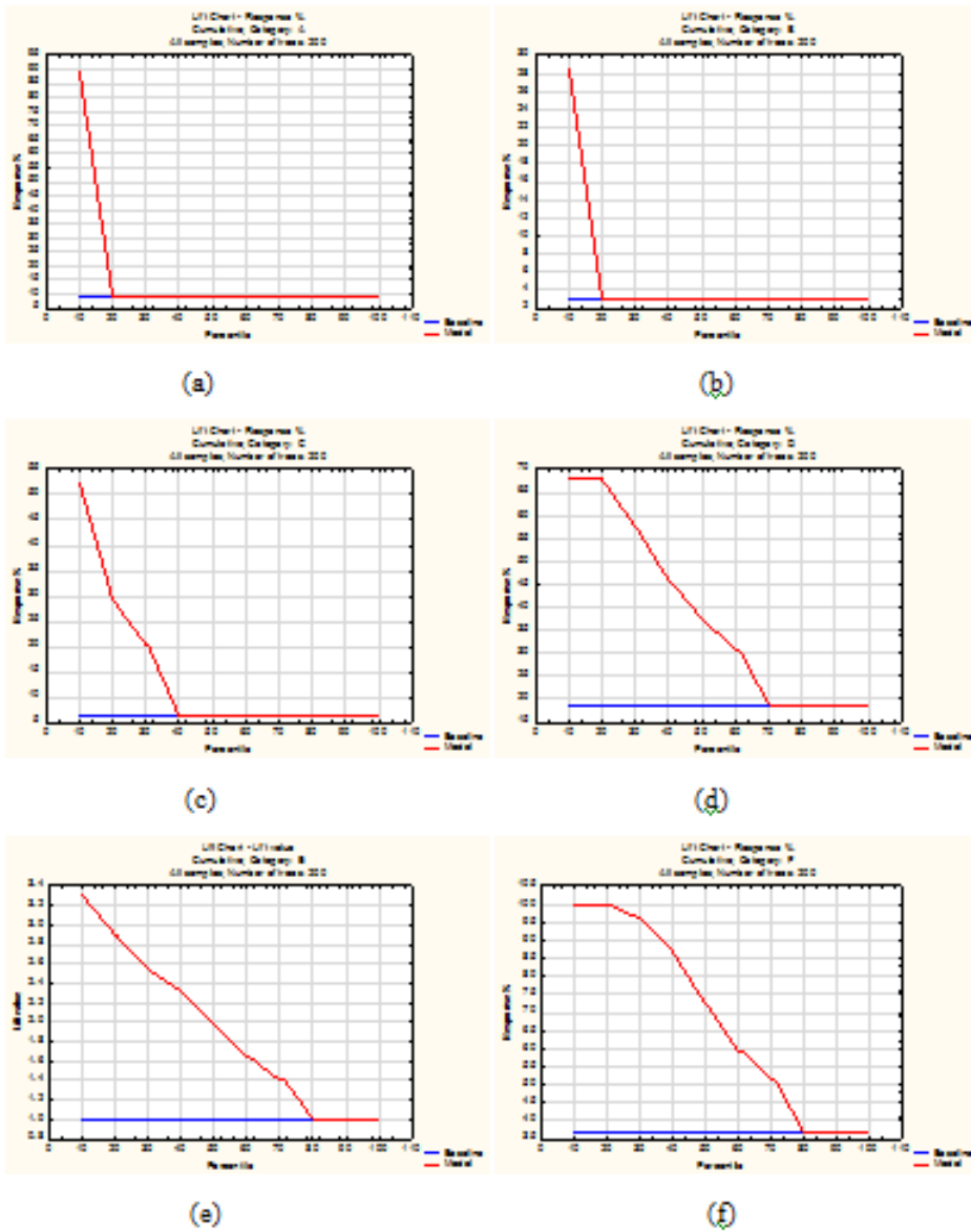
Figure 7. Lift Chart of CGPA with Random Forest
