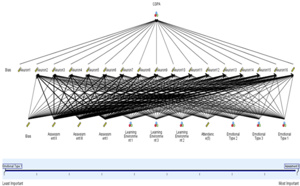
Figure 3. Neural Network Training with MLP
