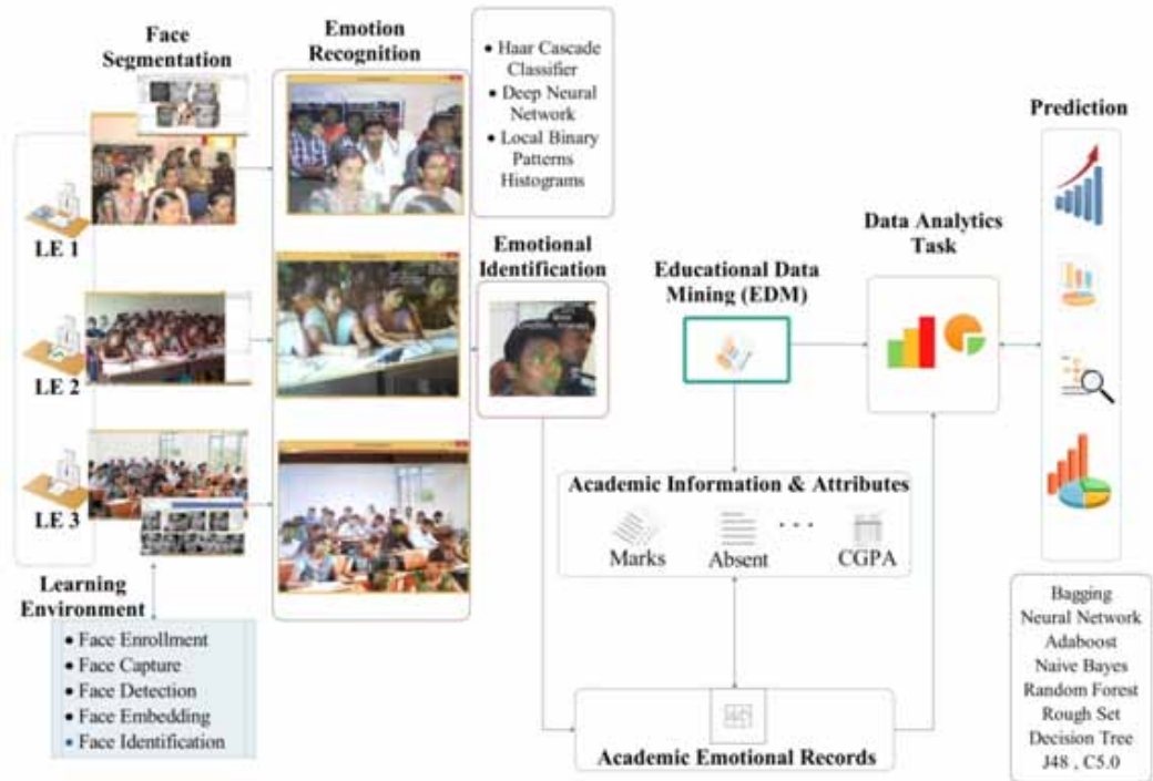
Figure 1. Emotion recognition in the learning environment
