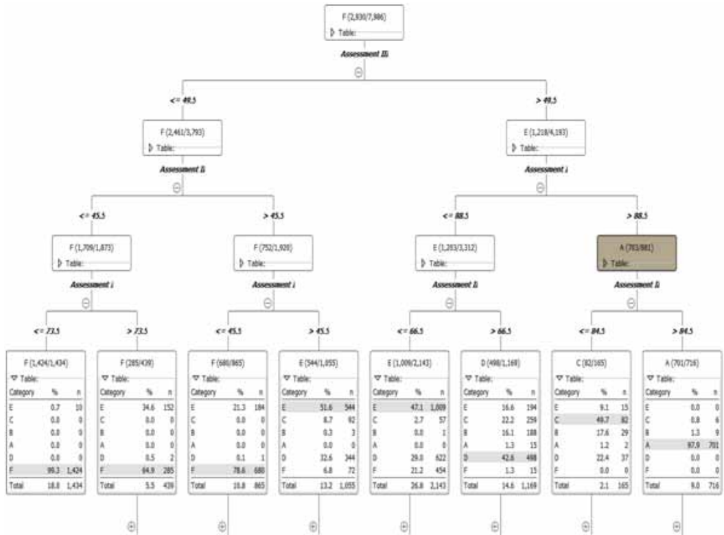
Figure 8. Decision Tree generated from Random forest
