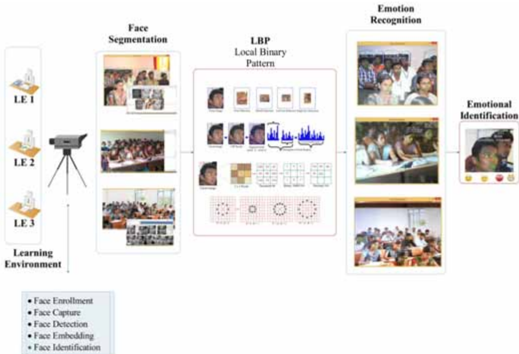
Figure 4. LBP features in Face Emotion estimator models
