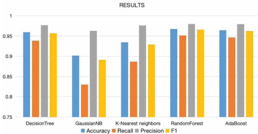
Figure 7. Traditional machine learning model evaluation results
