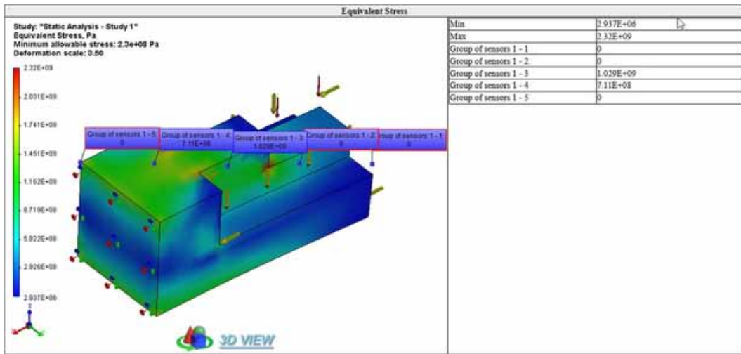
Figure 2. Equivalent Stress.
