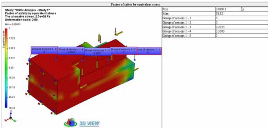
Figure 3. The factor of safety by equivalent stress.
