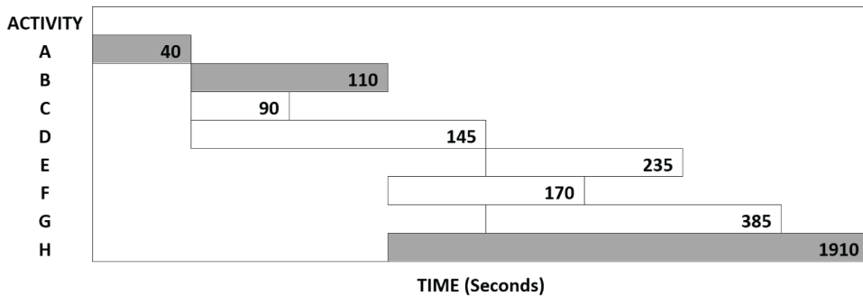
Figure 3. Gantt chart of the aircraft ground handling operations schedule
