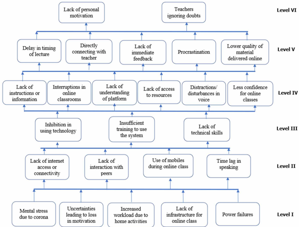
Figure 5. Final Graph Interpretive Structural Model (ISM)
