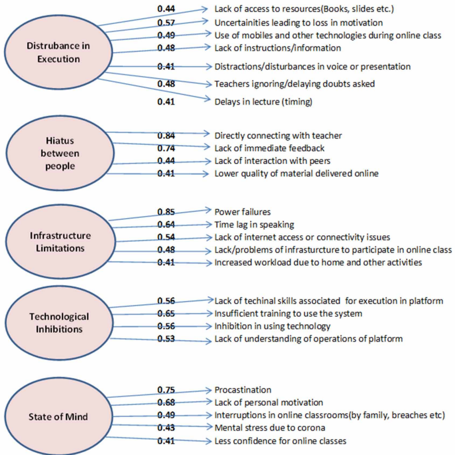
Figure 1. Model diagram using EFA
