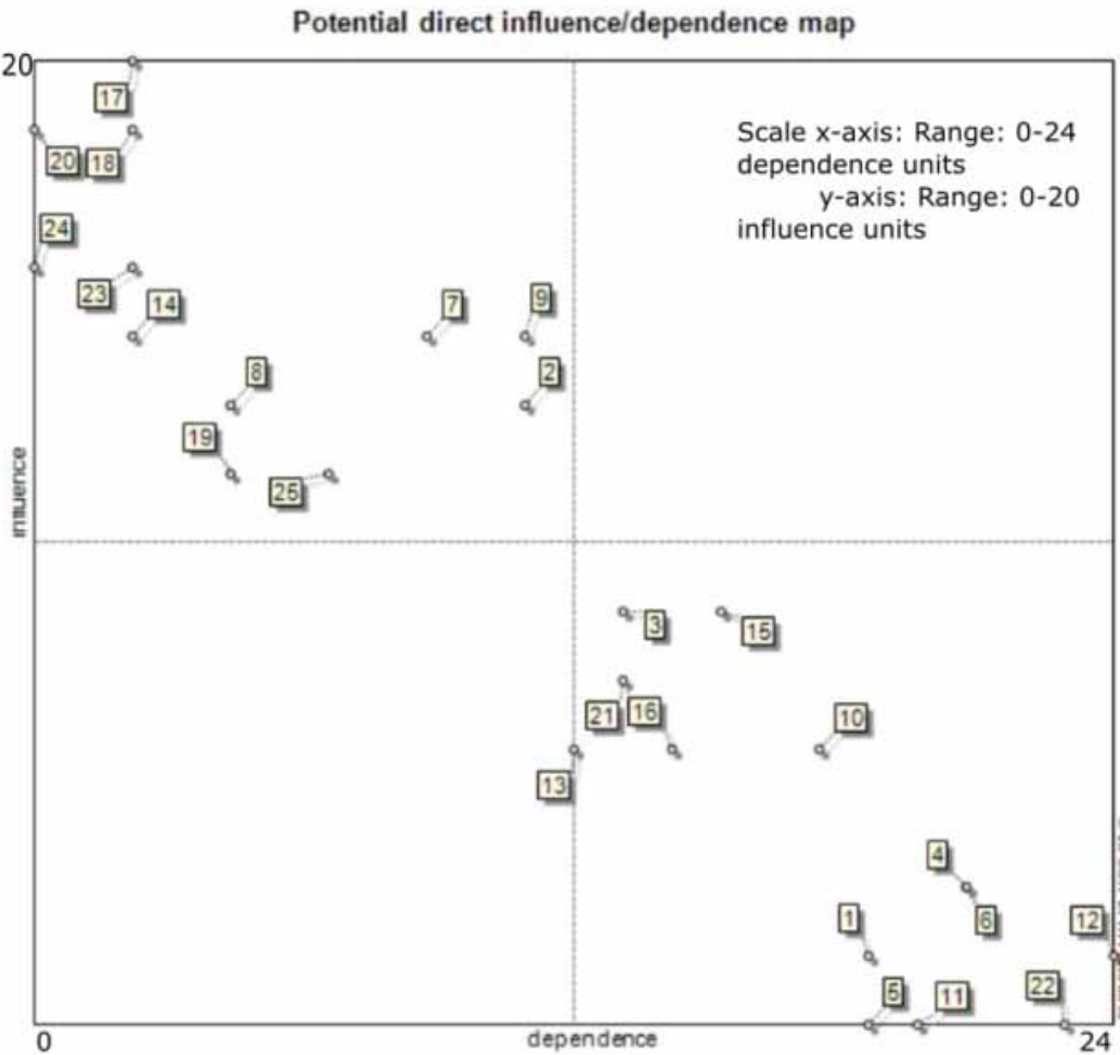
Figure 4. Influence and dependence map
