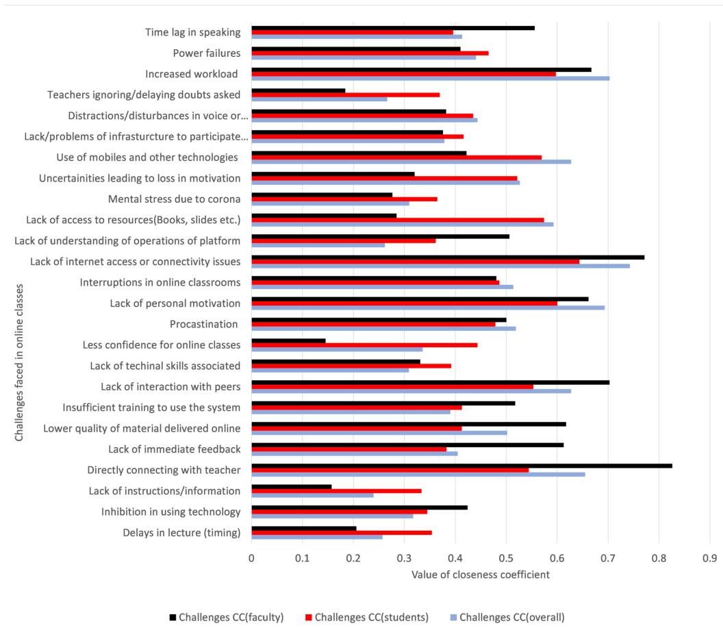
Figure 8. Closeness coefficients and rankings
