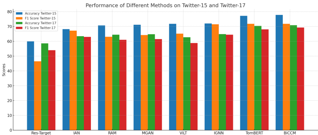
Figure 2. Experimental results of model ablation
