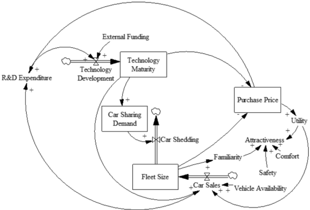
Figure 1. High level overview of the base model (adapted from Figure 2 of Nieuwenhuijsen et al. (2018))
