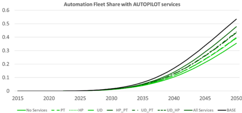
Figure 10. Shares of L4 + 5 vehicles with different AUTOPILOT services available (PT: Platooning; HP: Highway Pilot; UD: Urban Driving)
