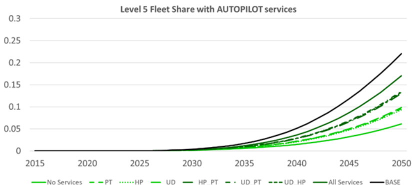
Figure 11. Shares of L5 vehicles with different AUTOPILOT services availability (PT: Platooning; HP: Highway Pilot; UD: Urban Driving)
