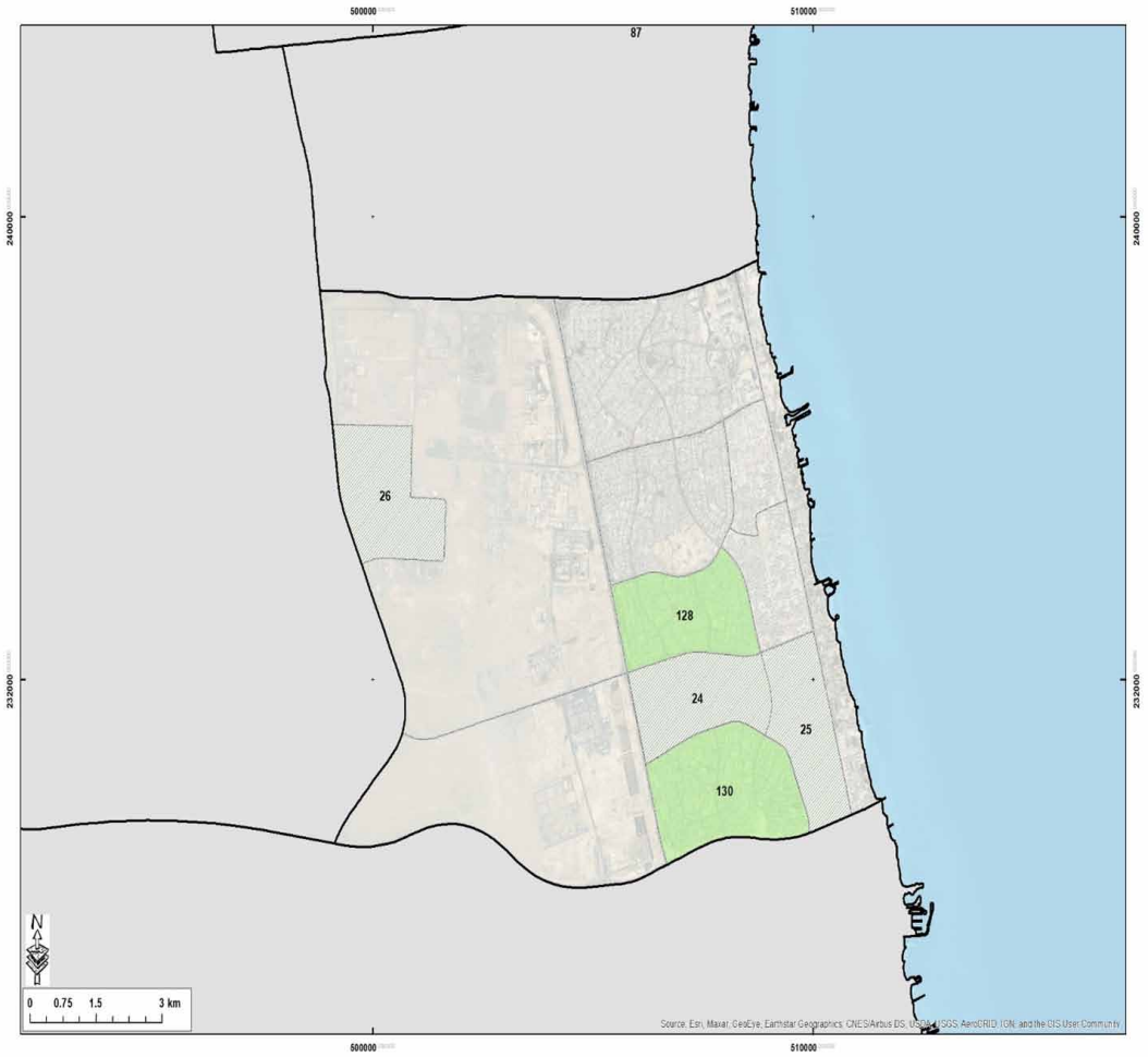
Figure 9. Optimal firefighting stations for Mubarak Al-Kabir
