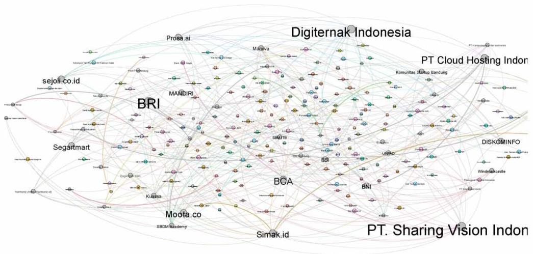
Figure 5. The eigencentality network structure Source: The authors
