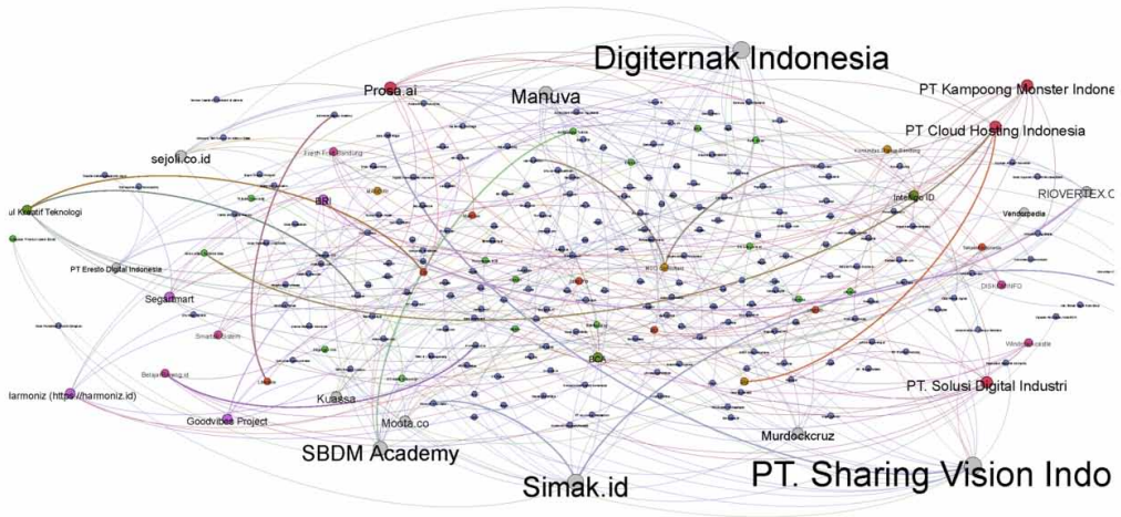
Figure 2. The degree centrality network structure Source: The authors
