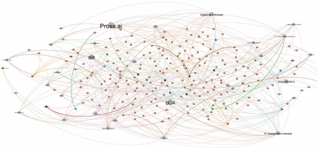
Figure 4. The betweenness centrality network structure Source: The authors
