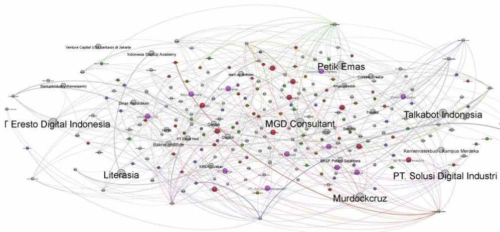
Figure 3. The closeness centrality network structure Source: The authors
